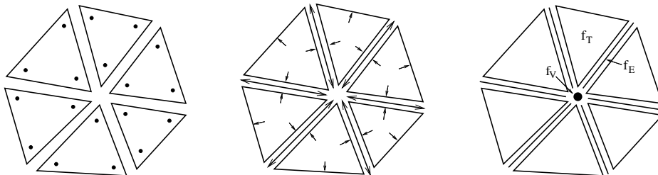
FIGURE 4. Distributional finite element spaces in the sequence (3.7). The arrows along the edges represent the edge and the vertex terms in (3.8).
